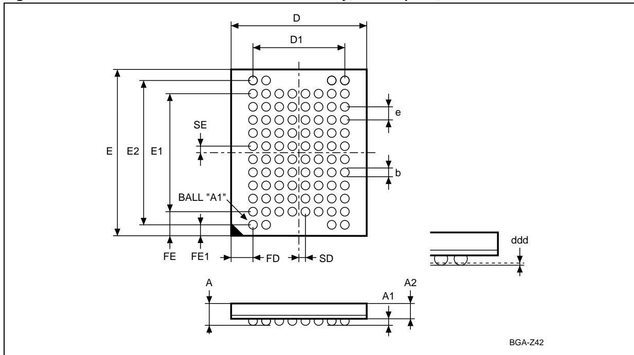
Figure 7. Stacked TFBGA88 8x10mm - 8x10 ball array, 0.8mm pitch, Bottom View Outline
